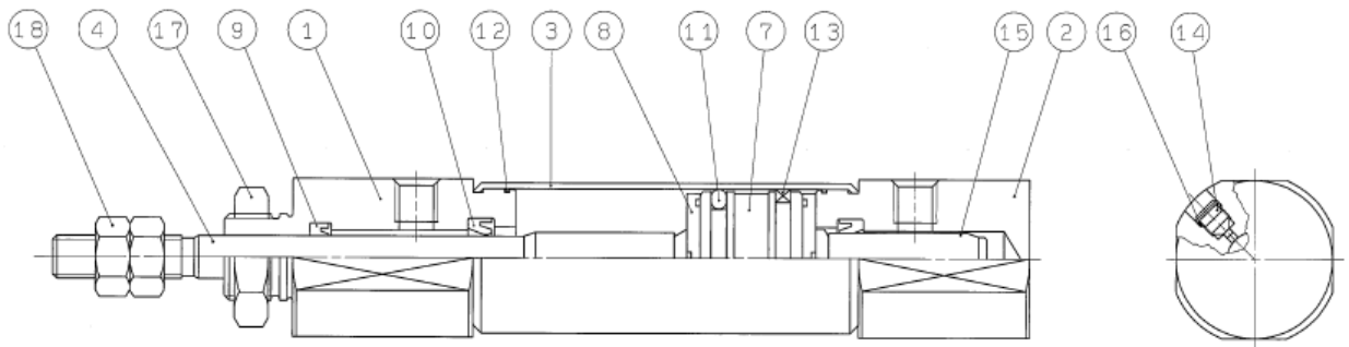
CJ2B10~16-*AZ
