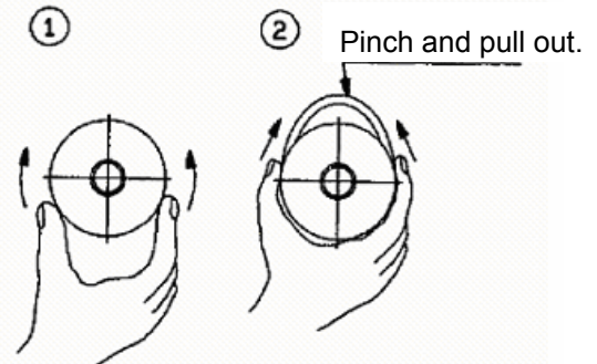
Fig. 7 How to remove piston seal
