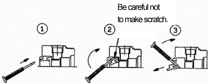
Fig. 6 How to remove rod seal
