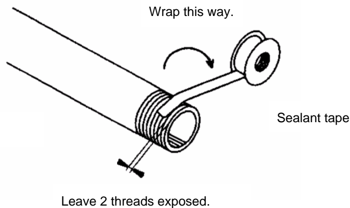
Fig. 2 Sealant tape
