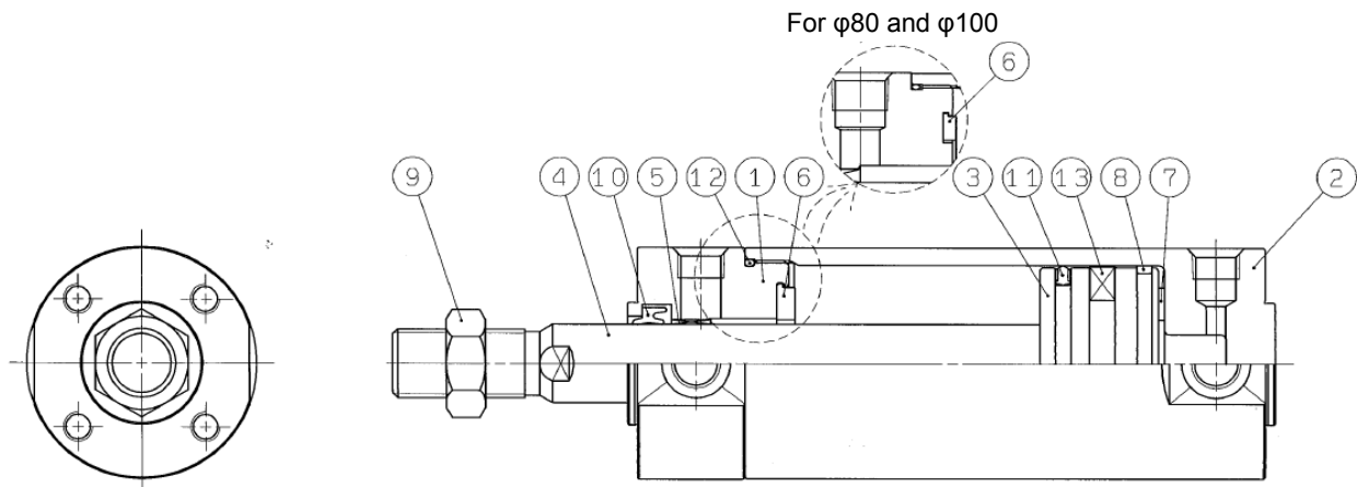
Fig. 12 Standard product: Double acting/single rod
