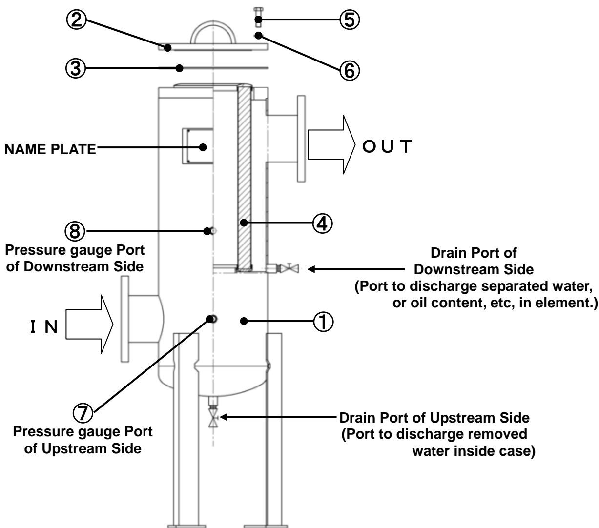
Fig. 1 Construction
