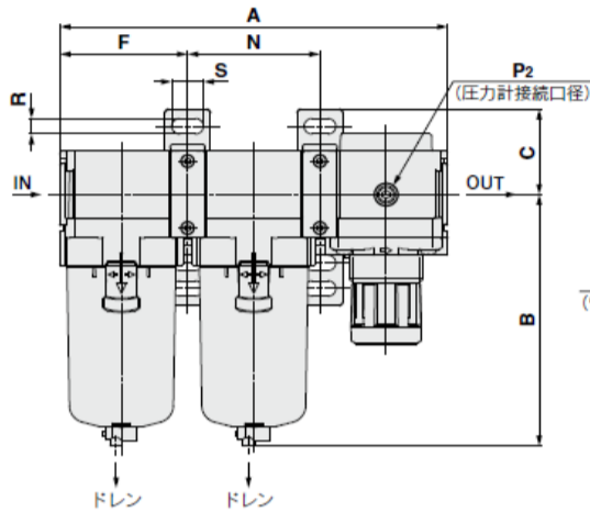
AC40C-D
