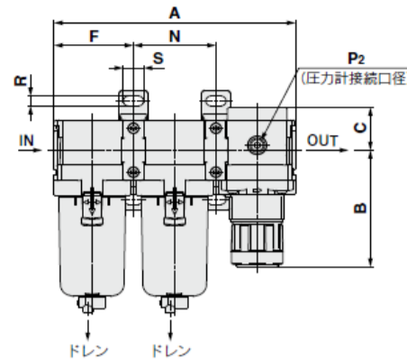
AC30C-D
