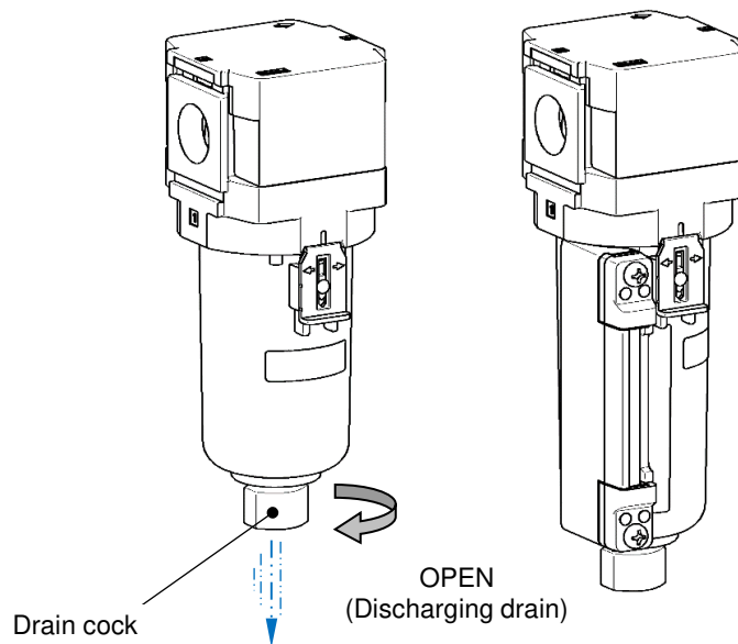
AFG30-D / AFG40-D: Drain cock (rotation type) (Metal bowl / Metal bowl with level gauge)
