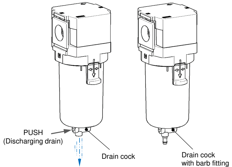
AFG30-D / AFG40-D: Drain cock (rotation type) (Metal bowl / Metal bowl with level gauge)
