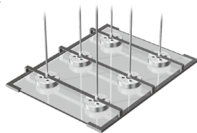
When using multiple non-contact grippers
