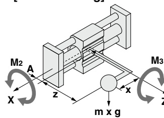
[Wall mounting]
